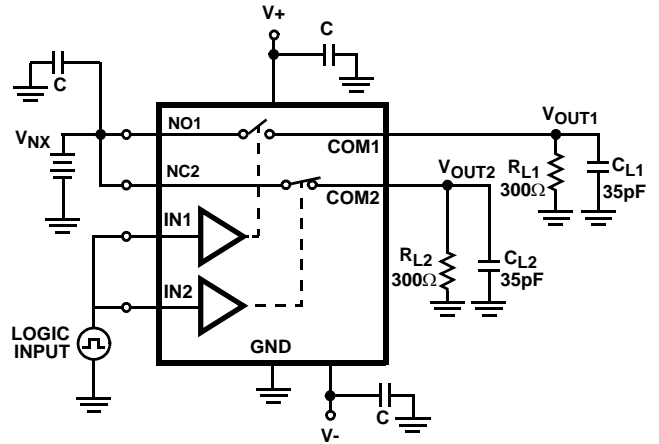
FIGURE 3B. TEST CIRCUIT C_L includes fixture and stray capacitance. Reconfigure accordingly to test SW3 and SW4.
