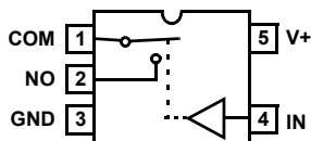
ISL84715 (SC70) TOP VIEW
