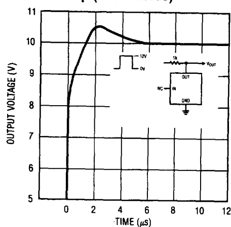
Start-Up (Shunt Mode)
