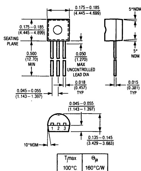
Z Package, 3 Lead TO-92 Plastic
