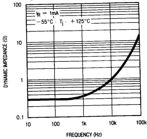
Dynamic Impedance
