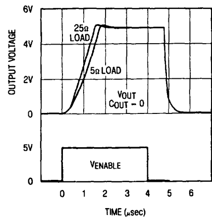
Switching Characteristics
