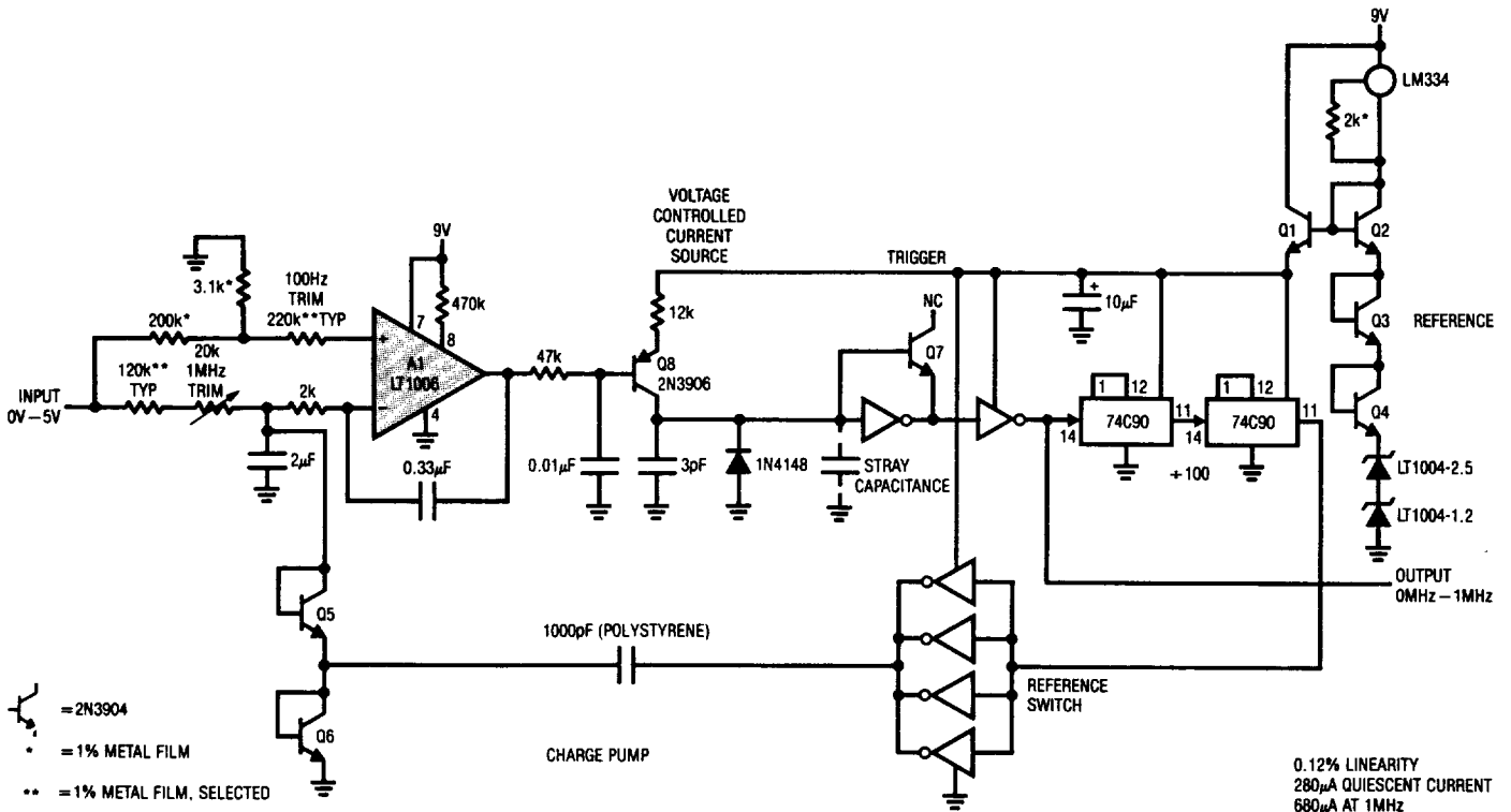
Micropower 1MHz V-F Converter
