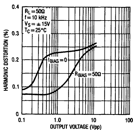
Total Harmonic Distortion
