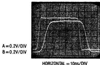
Figure A. Waveforms Using LT1010
