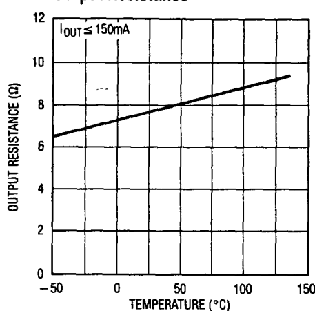
Output Resistance
