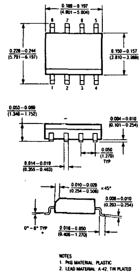
SO Package 8-Lead Plastic SOIC
