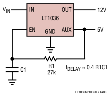
Delayed Power-Up
