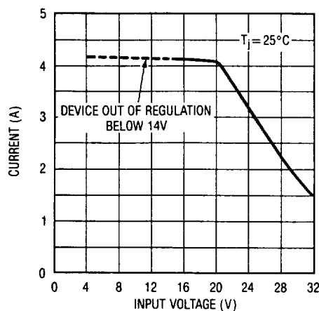
Maximum Available Load Current, 12V Output
