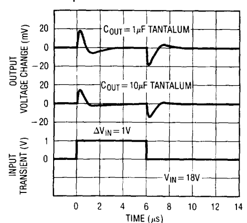
Line Transient Response, 12V Output
