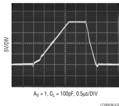
LT1055 Large-Signal Response
