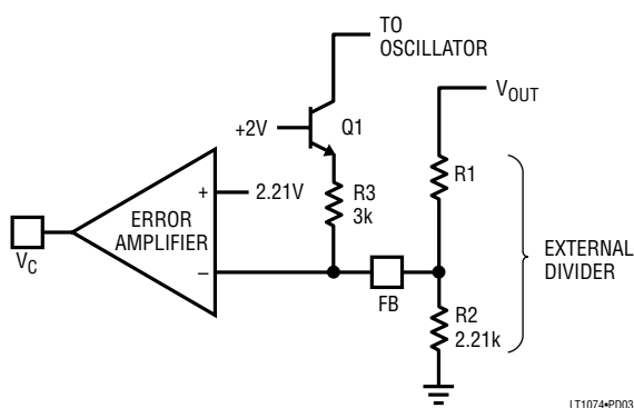
Figure 3. Frequency Shifting
