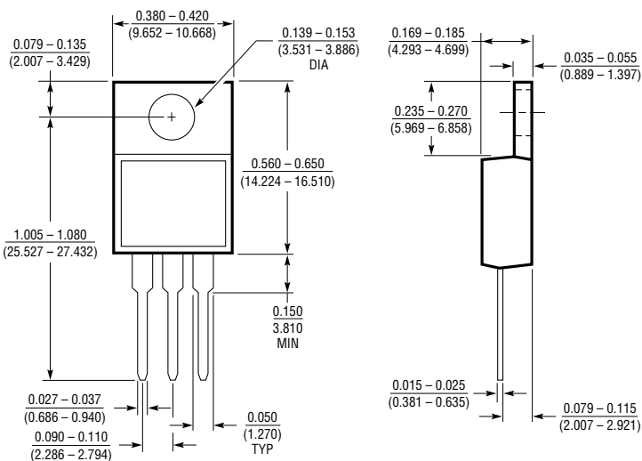
T Package 3-Lead Plastic TO-220
