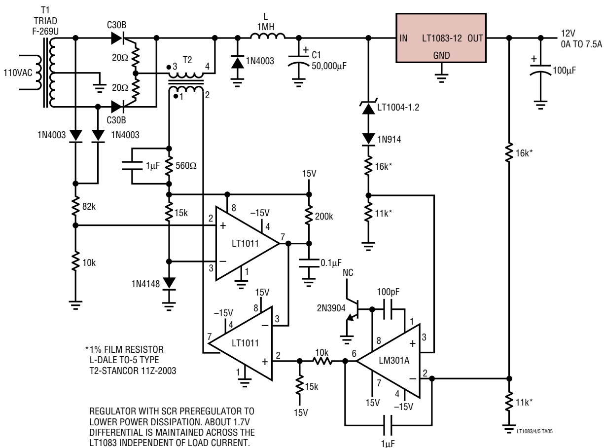
7.5A Regulator
