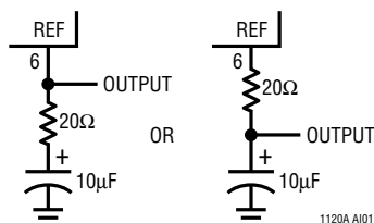
Figure 1. Bypassing Reference
