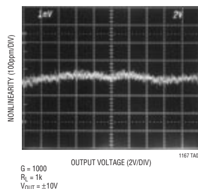
Gain Nonlinearity
