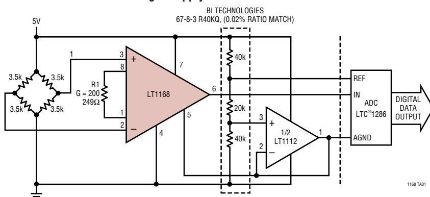
Single Supply* Pressure Monitor
