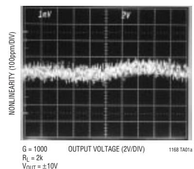
Gain Nonlinearity
