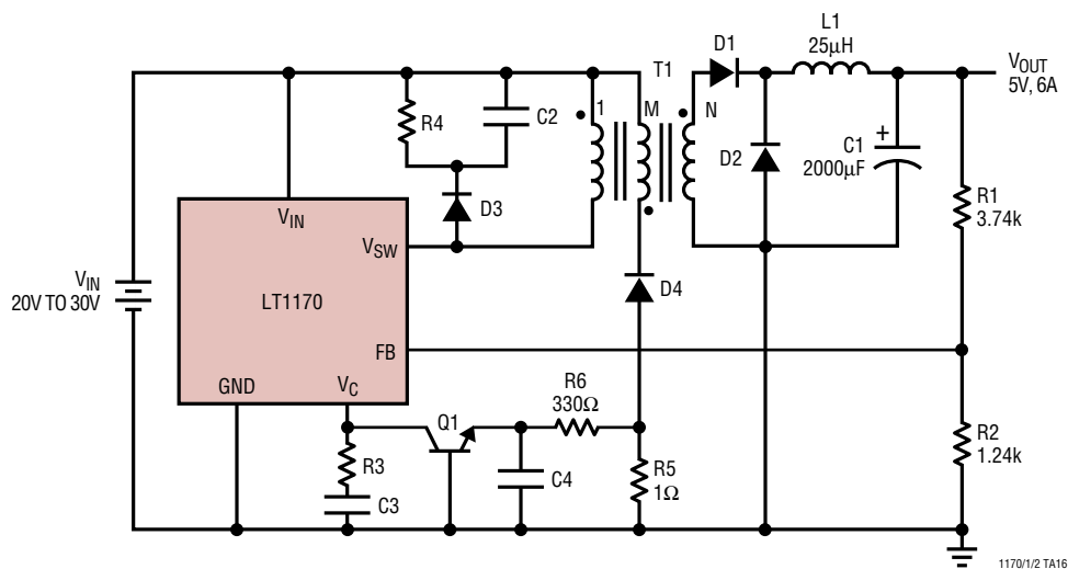
Forward Converter
