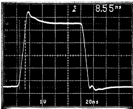
A_V = +1, C_L = 10\text{pF} SCOPE PROBE LT1190 - TPC22
