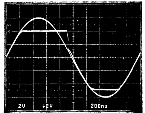
A_V = -1, V_{IN} = 12\text{Vp-p} LT1190 - TPC23
