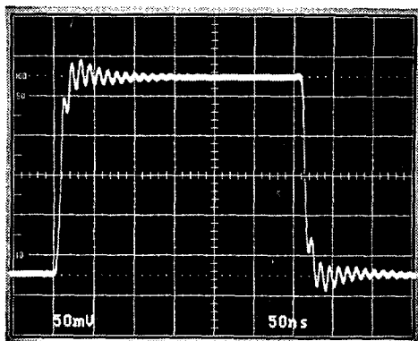
A_V = -1 , IN DEMO BOARD, C_L = 50\text{pF}
