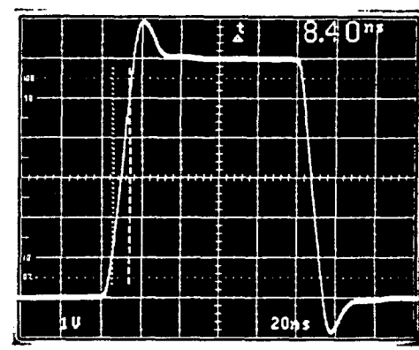
A_v = -1 , C_L = 10 pF SCOPE PROBE
