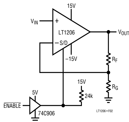
Figure 2. Shutdown Interface
