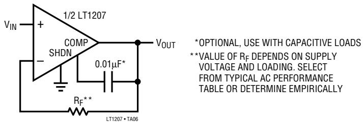
Buffer A_V = 1
