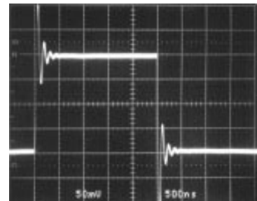
Small Signal, A_V = -1 , C_L = 1,000pF
