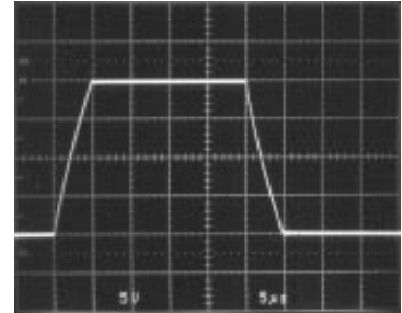
Large Signal, A_V = 1 , C_L = 10,000pF
