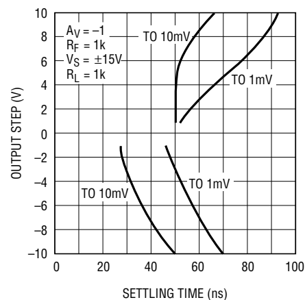
Inverting Amplifier Settling Time vs Output Step
