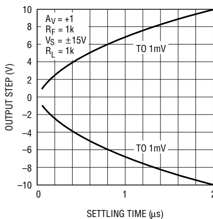
Noninverting Amplifier Settling Time to 1mV vs Output Step
