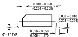
S8 Package 8-Lead Plastic SOIC
