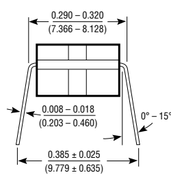
J8 Package 8-Lead Ceramic DIP
