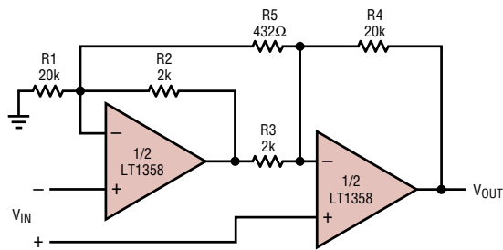
Instrumentation Amplifier
