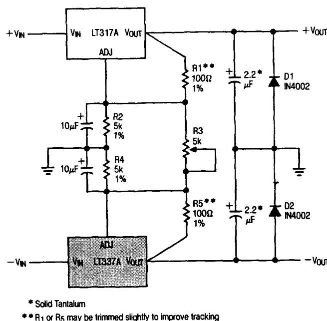
Dual Tracking Supply \pm 1.25\text{V} to \pm 20\text{V}
