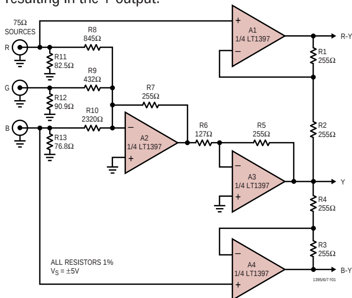
Figure 1. Buffered RGB to Color-Difference Matrix
