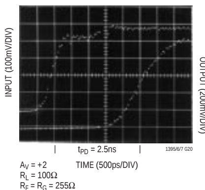
Propagation Delay
