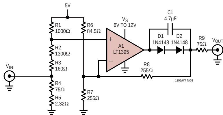
Figure 3. Single Supply RGB Video Amplifier (1 of 4 Channels)
