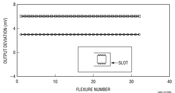
Figure 8b. Same Two LT1460S8-10s in Figure 7b, but With Slots
