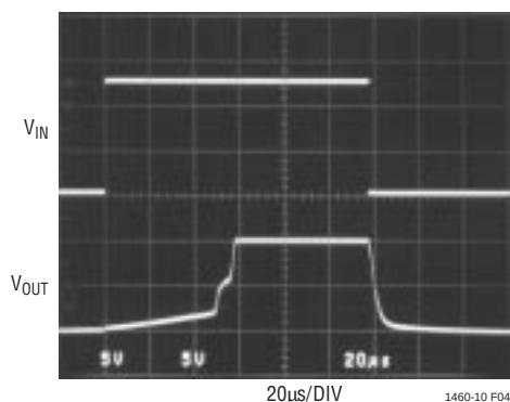
Figure 4. C_{IN} = 0
