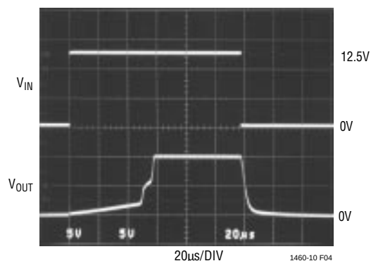
Figure 4. C_{IN} = 0
