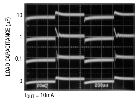
Transient Responses
