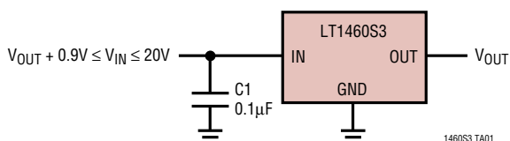
Basic Connection
