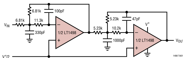
Single Supply 100kHz 4th Order Butterworth Filter
