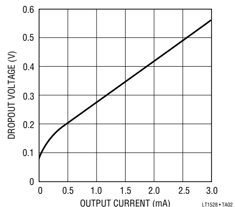
Dropout Voltage
