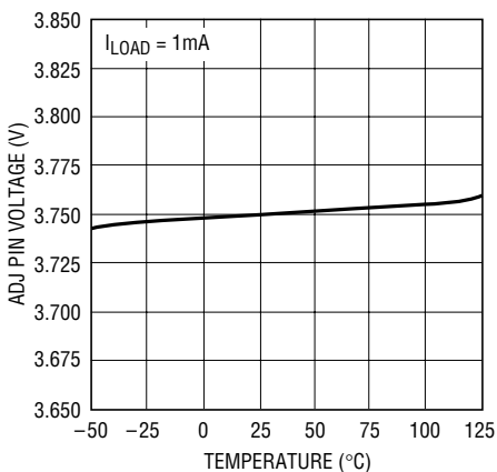
LT1529 ADJ Pin Voltage
