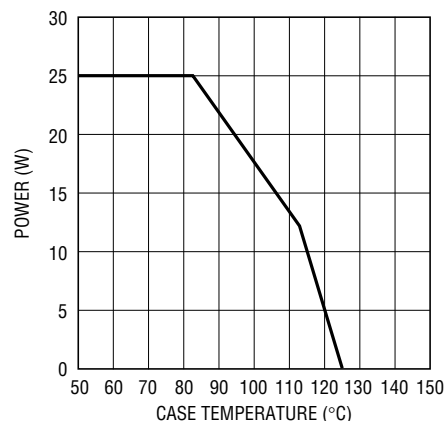
LT1584 Maximum Power Dissipation*
