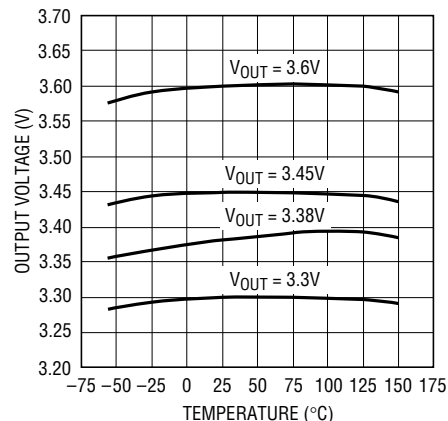
LT1584/5/7-3.XX Output Voltage vs Temperature
