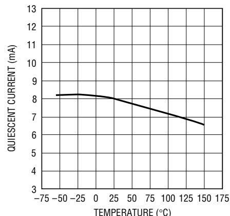
LT1584/5/7-3.XX Quiescent Current vs Temperature
