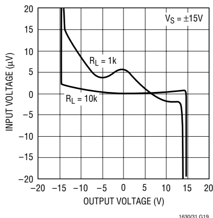
Open-Loop Gain
