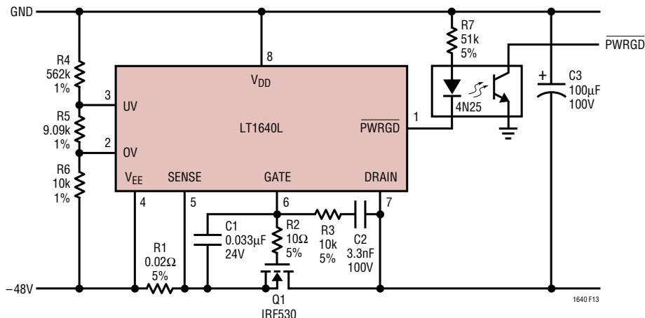
Figure 13. Using PWRGD to Drive an Optoisolator
