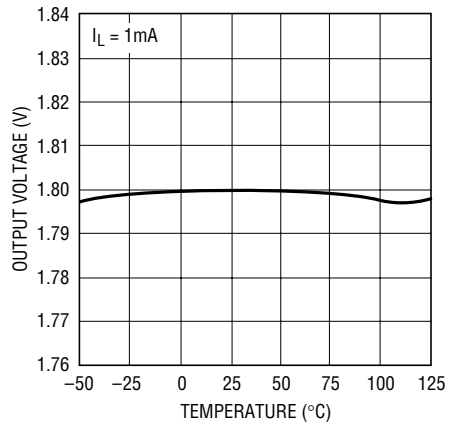
LT1761-1.8 Output Voltage
