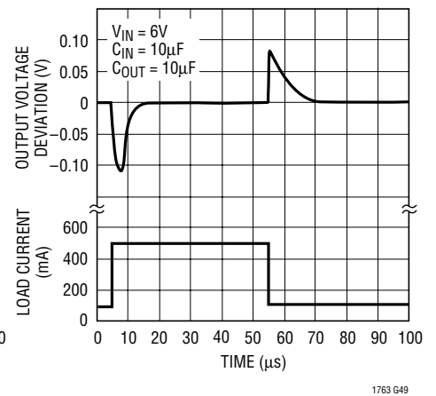
LT1763-5 Transient Response C_{BYP} = 0.01µF
