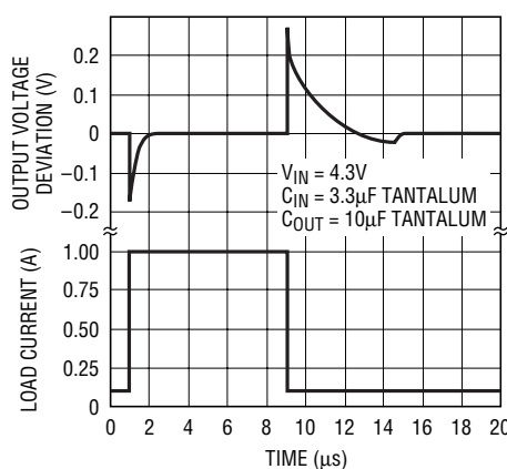
LT1764-3.3 Transient Response
