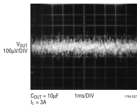
LT1764-3.3 10Hz to 100kHz Output Noise
