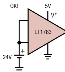
INPUT OVERVOLTAGE
