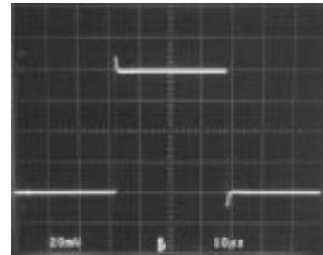
Small-Signal Response
