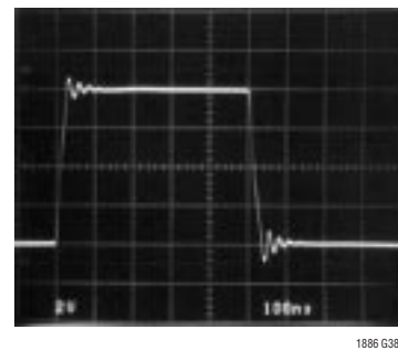
Large-Signal Transient, A_V = 10 , C_L = 1000pF
