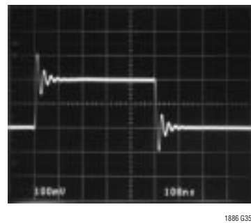
Small-Signal Transient, A_V = 10 , C_L = 1000pF
