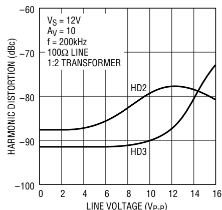
ADSL Modem Line Driver Distortion
