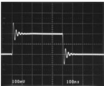
Small-Signal Transient, A_V = 10 , C_L = 1000pF
