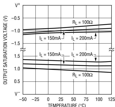
Output Saturation Voltage vs Temperature, V_S = \pm 6V
