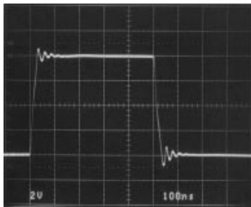
Large-Signal Transient, A_V = 10 , C_L = 1000pF
