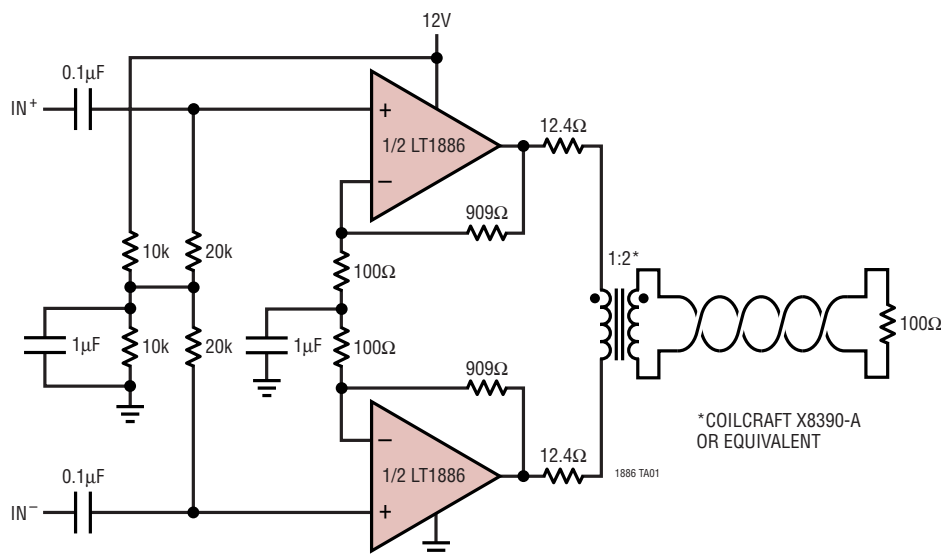
Single 12V Supply ADSL Modem Line Driver
