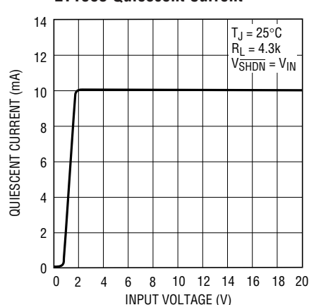
LT1963 Quiescent Current
