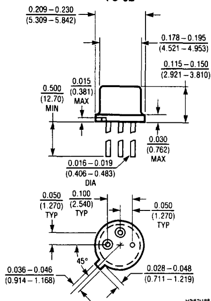
LT580 TO-52
