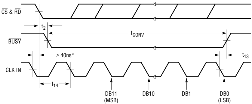
UNCERTAIN CONVERSION TIME FOR 30\text{ns} < t_{14} < 180\text{ns} *THE LTC1272 IS ALSO COMPATIBLE WITH THE AD7572 SYNCHRONIZATION MODES. SEE "DIGITAL INTERFACE" TEXT.
