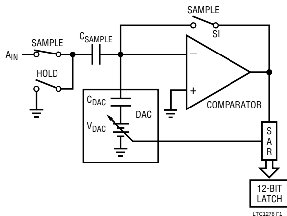
Figure 1. A_{IN} Input
