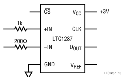
Figure 16. Overvoltage Protection for Inputs
