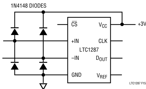
Figure 15. Overvoltage Protection for Inputs
