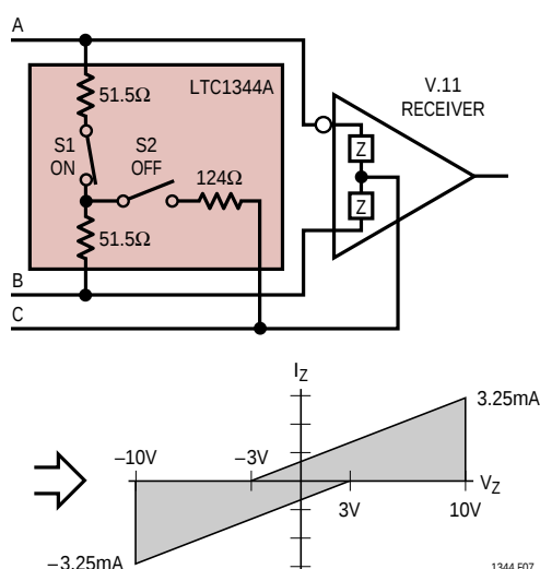
Figure 7. V.11 Interface Using the LTC1344A
